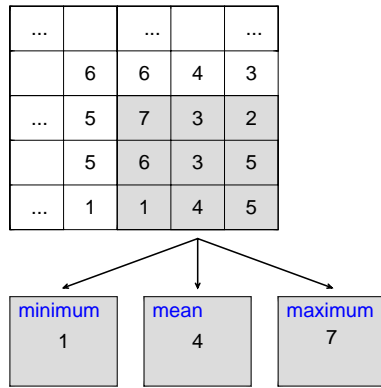
Fig. 4. Illustration of coarse-graining modes of the elevation model employing minimum, mean, and maximum. For an aggregation of 3×3 grid cells in the DEM (top) an example of the different resulting cell values (bottom) is displayed (with exemplary numbers).
